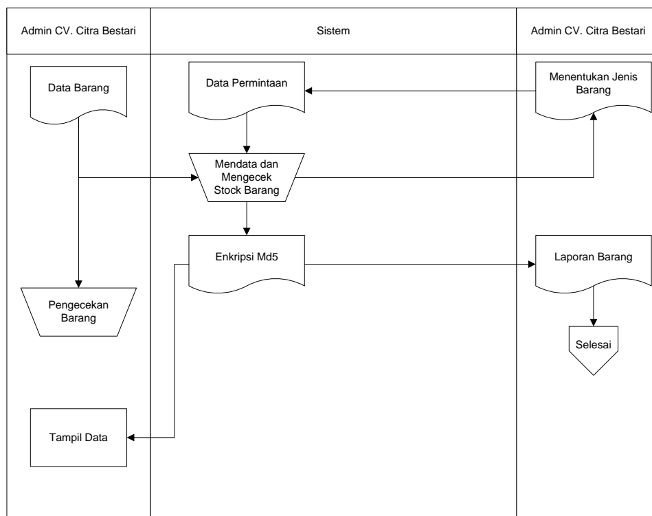
Gambar 3.2. Flowmap Usulan
