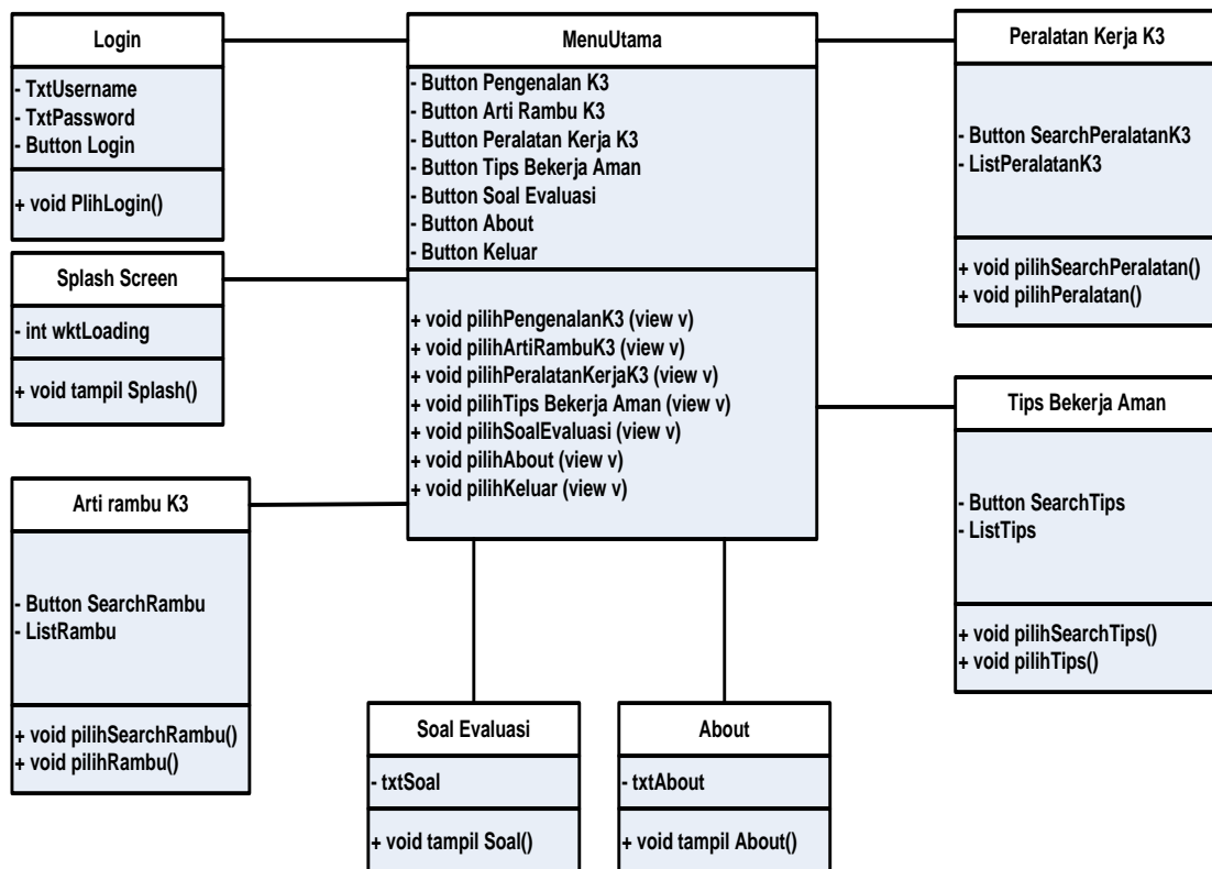
Gambar 3.6. Class Diagram
