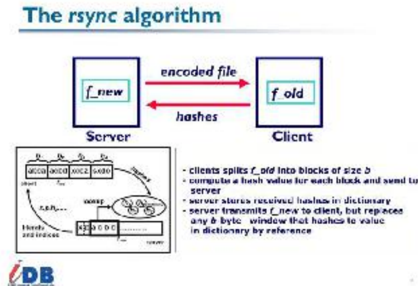
Gambar 2. 2 The rsync algorithm
