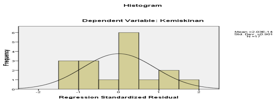
Gambar 4.3: histogram
