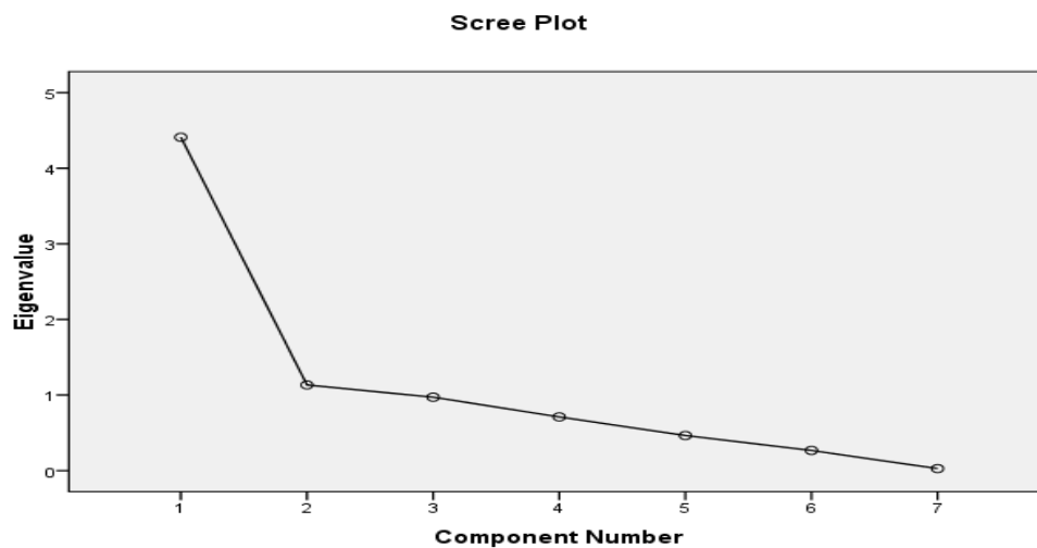
Gambar 4.1 scree plot
