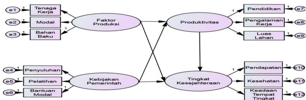
Gambar 2.1 : Kerangka Konseptual Structural Equation Modelling (SEM)
