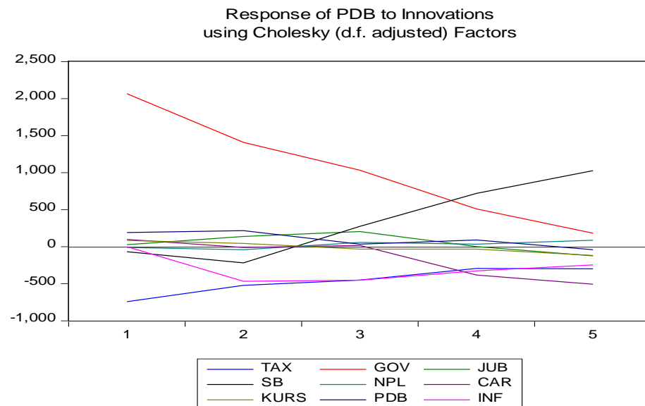
Gambar 4.18 Impulse Response Function of PDB
